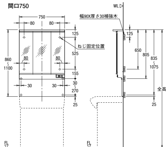
間口750
