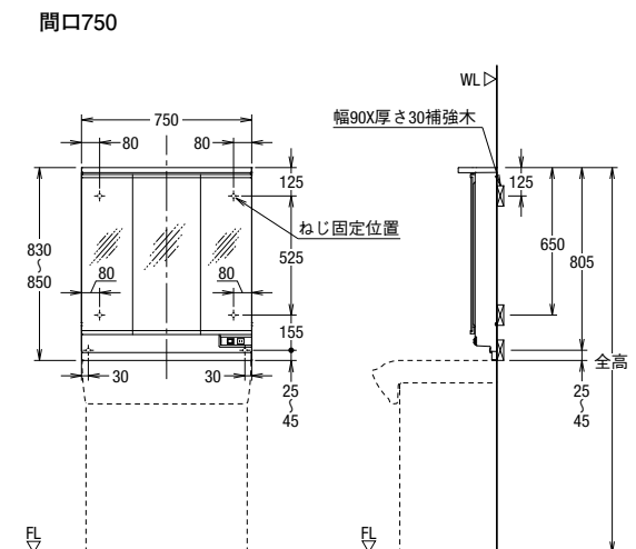
間口750
